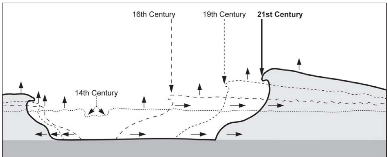
Figure 15. Lowland rofabard development 14th–21st century AD. Once rofabards have developed, small-scale lateral movements of the eroding face can result in large-scale sediment mobilization, a process enhanced by the thickening of the surviving soil profile (Fig. 14).
