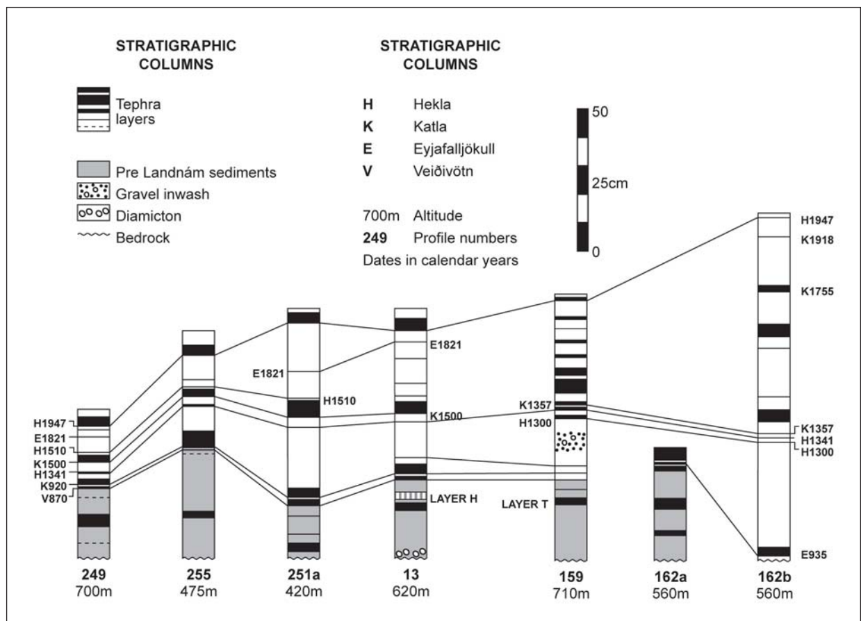
Figure 9. Tephra stratigraphy in upland profiles located on Figure 1. At the time of settlement soil profiles at these sites were less than 50 cm deep (Fig. 6).
