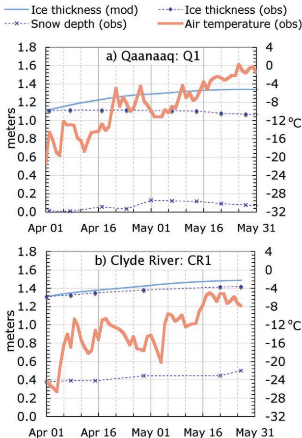
FIG. 4. Observed sea ice thickness compared with results of a 1D model driven by observed snow depths and air temperatures.
